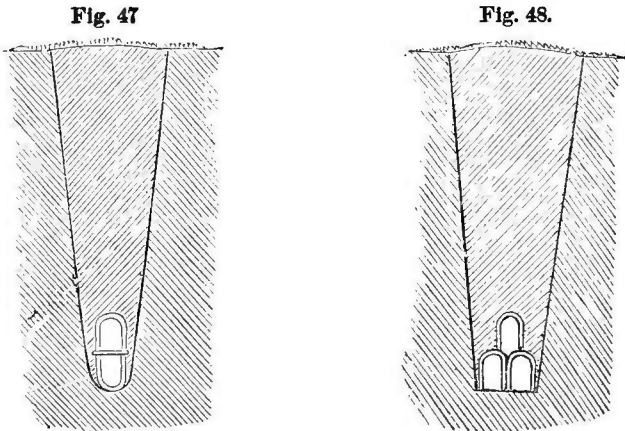
Main Drain of two or more Horse-shoe Tiles.
