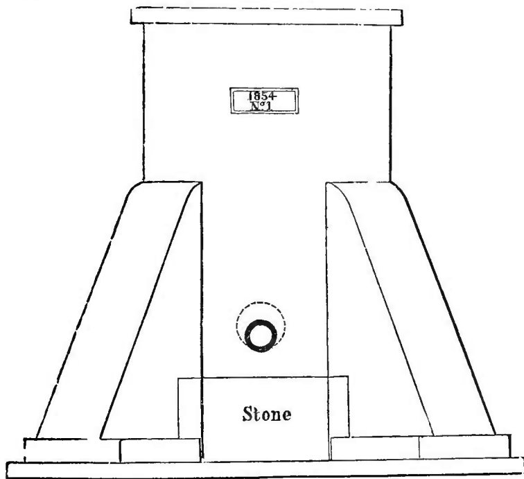
Fig. 38.—LARGE OUTLET.
