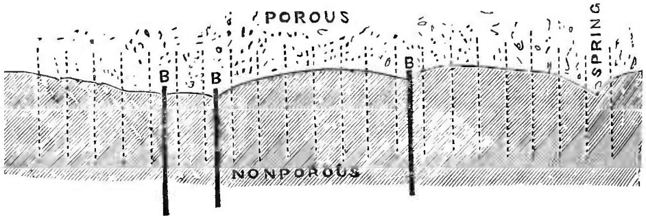
Fig. 85.—The vertical dotted lines show the position of parallel drains.
