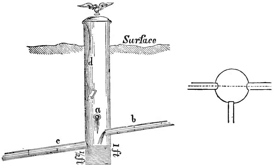
Figs. 45 & 46.—HOW TO PRESERVE A SPRING IN A DRAINED FIELD.
