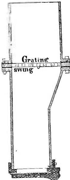
Fig. 40. — OUTLET PIPE WITH FLAP TO EXCLUDE FLOOD-WATER.
