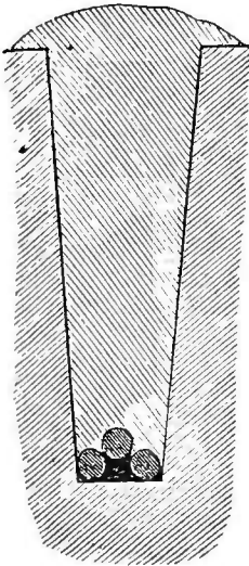
Fig. 17.—POLE-DRAIN.
