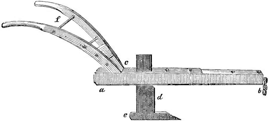
Fig. 13.—MOLE PLOW.
