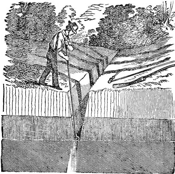
Fig. 83.—PIPE-LAYING.
