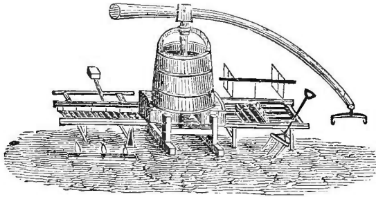
Fig. 53.—PRATT'S TILE MACHINE.
