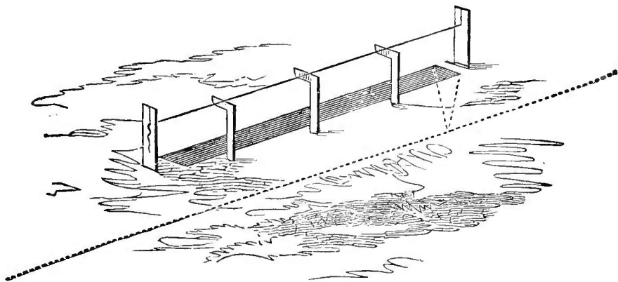
Fig. 59.—GRADING TRENCHES BY LINES.
