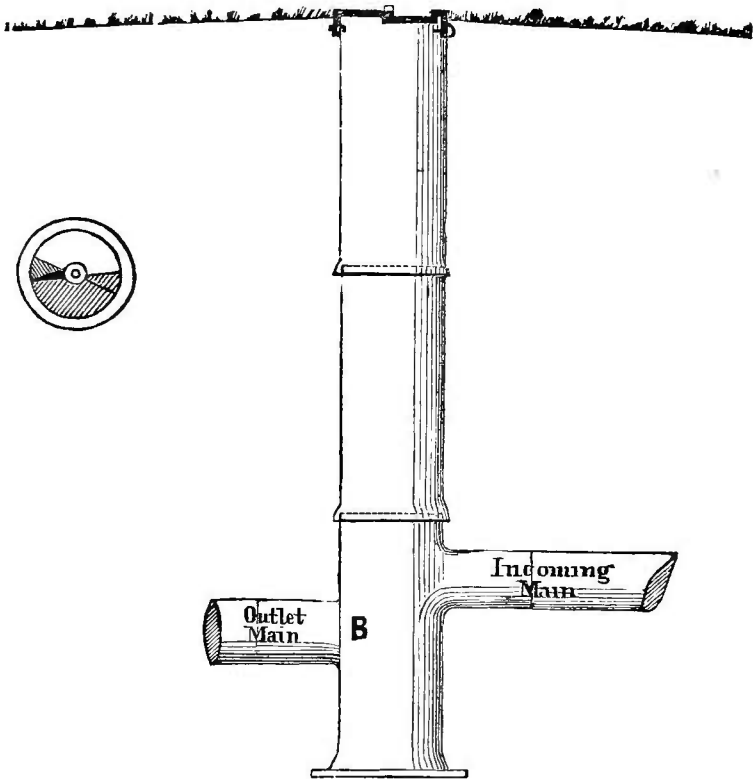
Figs. 43 & 44.—SMALL WELL, OR PEEP-HOLE, AND COVER
