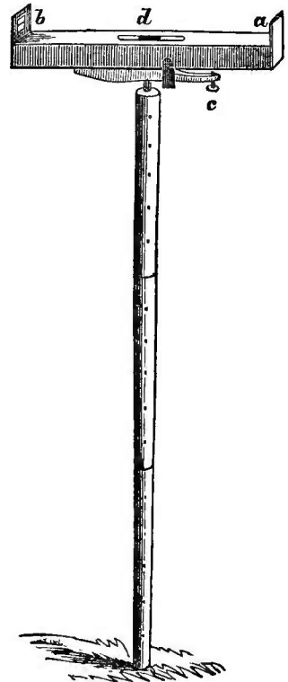
Fig. 56.—SPIRIT LEVEL.
