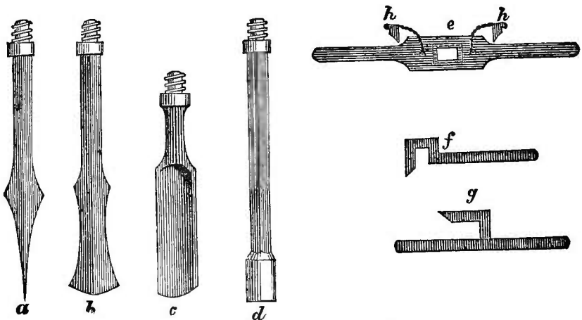
Fig. 87 —ELKINGTON'S DRAINING AUGER.
