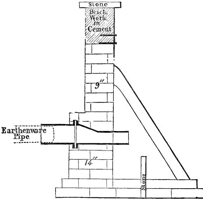
Fig. 89.—LARGE OUTLET.
