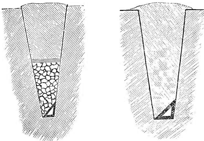
Fig. 24, 25.—STONE DRAINS.
