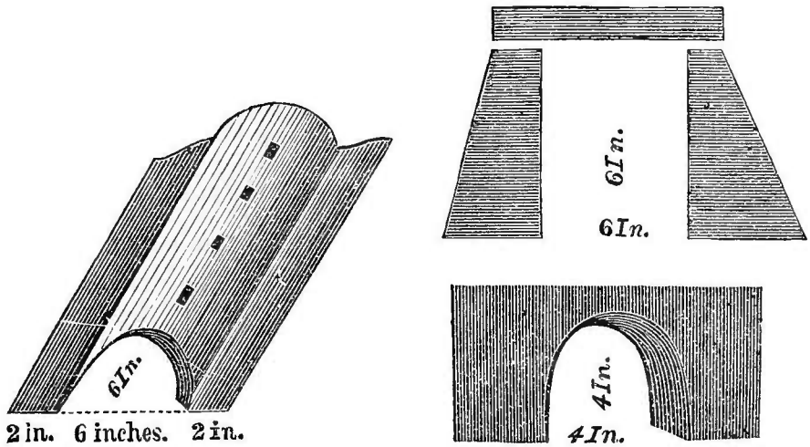
Fig. 26.—DRAINING-BRICKS.
