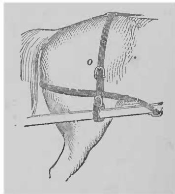
BREECHEN AND KICKING-STRAP UNITED.
