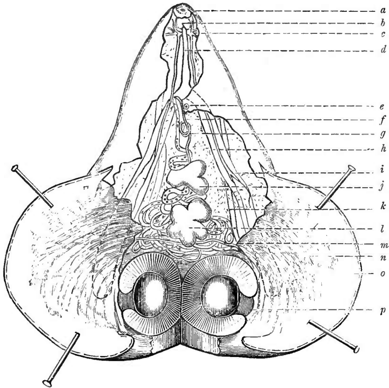
FIG. 6.—The human amphistome ( Amphistoma hominis ). Longitudinal section. a , Oral sucker ; b , pharyngeal bulb ; c , nerve ganglia ; d , cesophagus ; e , genital pore ; f , vagina ; g , ductus ejaculatorius ; h , ventral nerve cords ; i , intestinal canal ; j , upper testis ; k , water vessel ; l , lower testis (ovary according to Lewis) ; m , principal ducts of the vitellarium ; n , branches of the vitellary ducts ; o , ventral pouch or bursa ; p , caudal sucker. Magnified 12 diameters. After Lewis.
