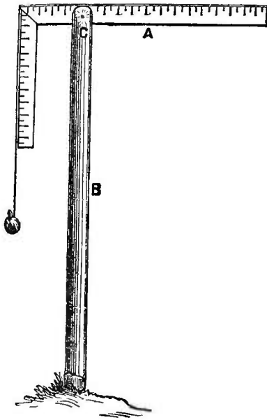
Fig. 55.—SQUARE AND PLUMB-LEVEL.
